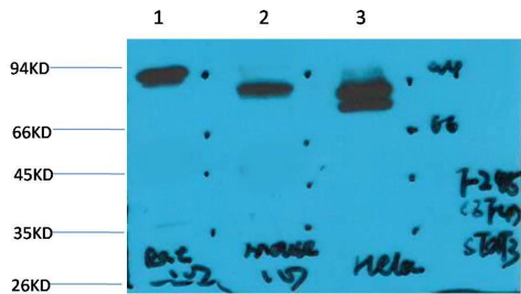
Western blot analysis of 1) Rat Heart Tissue, 2) Mouse Heart Tissue, 3) HeLa with STAT3 Mouse mAb diluted at 1:2,000.
